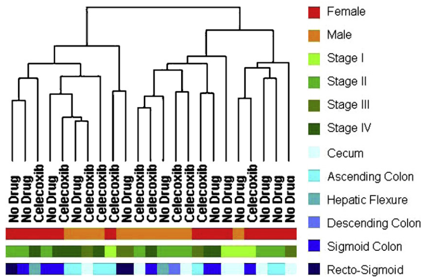
Fig. 1 – Clustering of gene expression in colorectal adenocarcinoma patients. Unsupervised hierarchical clustering was performed on all samples using 10,083 genes with a normalised expression standard deviations greater than 0.04. The dendrogram indicates that the samples do not cluster based solely on any of the recorded phenotypic characteristics.
